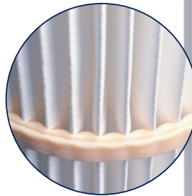
iPLAS is available only with BHA pleated filter elements.
